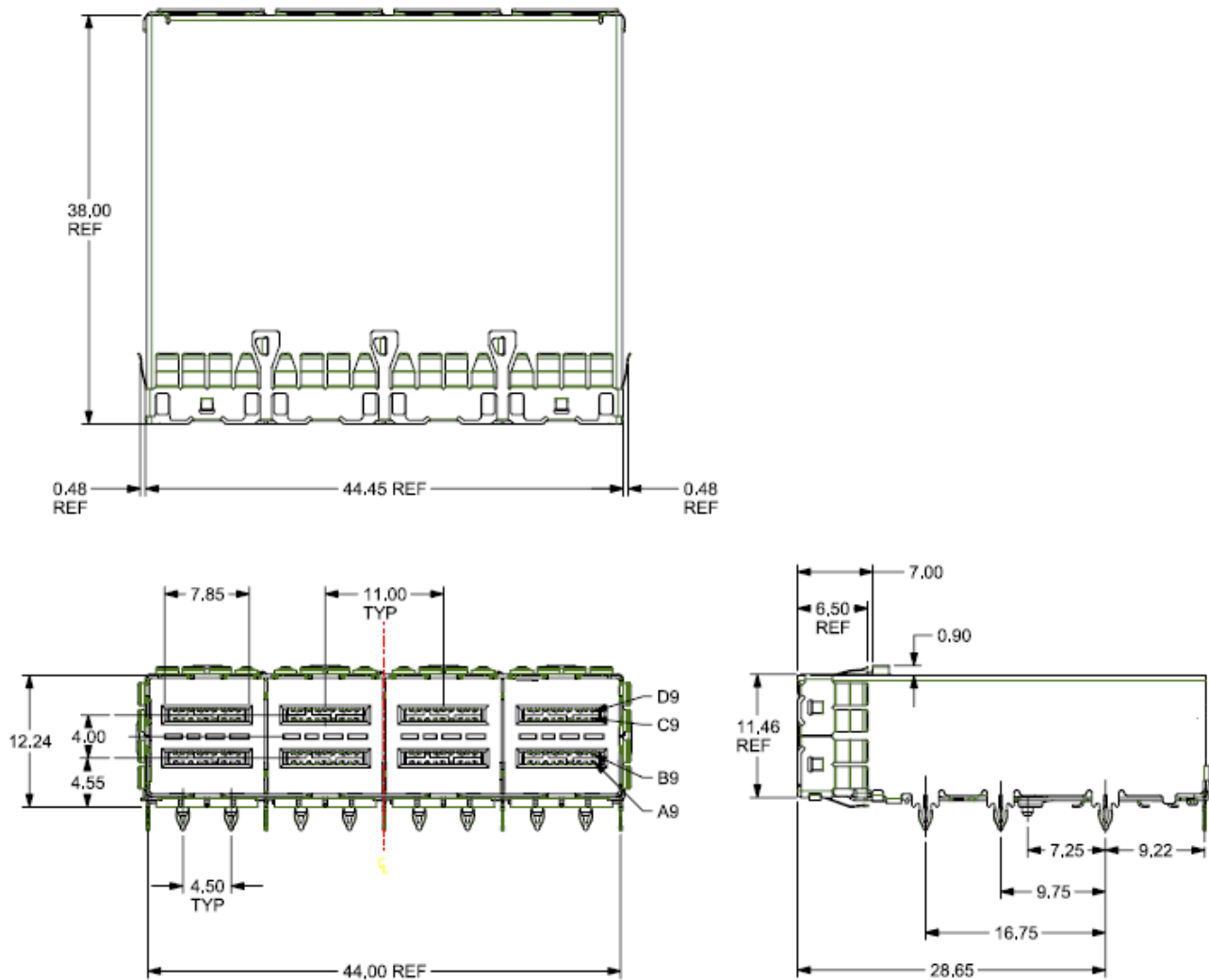
Figure 5-11 Cage for 1x4 SMT Connector
