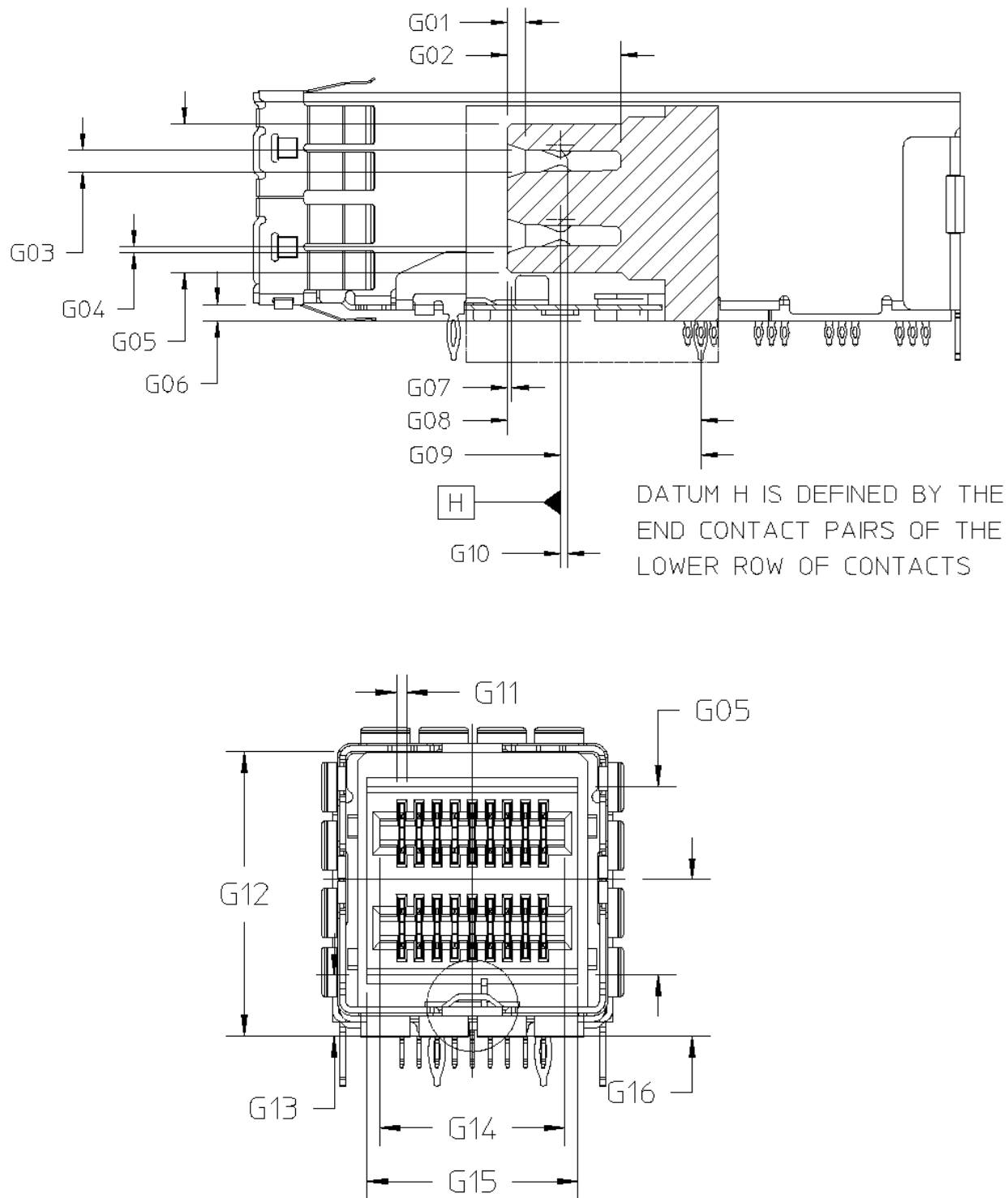
Figure 5-4 Receptacle Contact Locations
