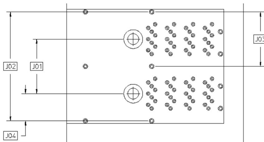
Figure 5-13 1x2 Receptacle Press Fit Footprint Option
