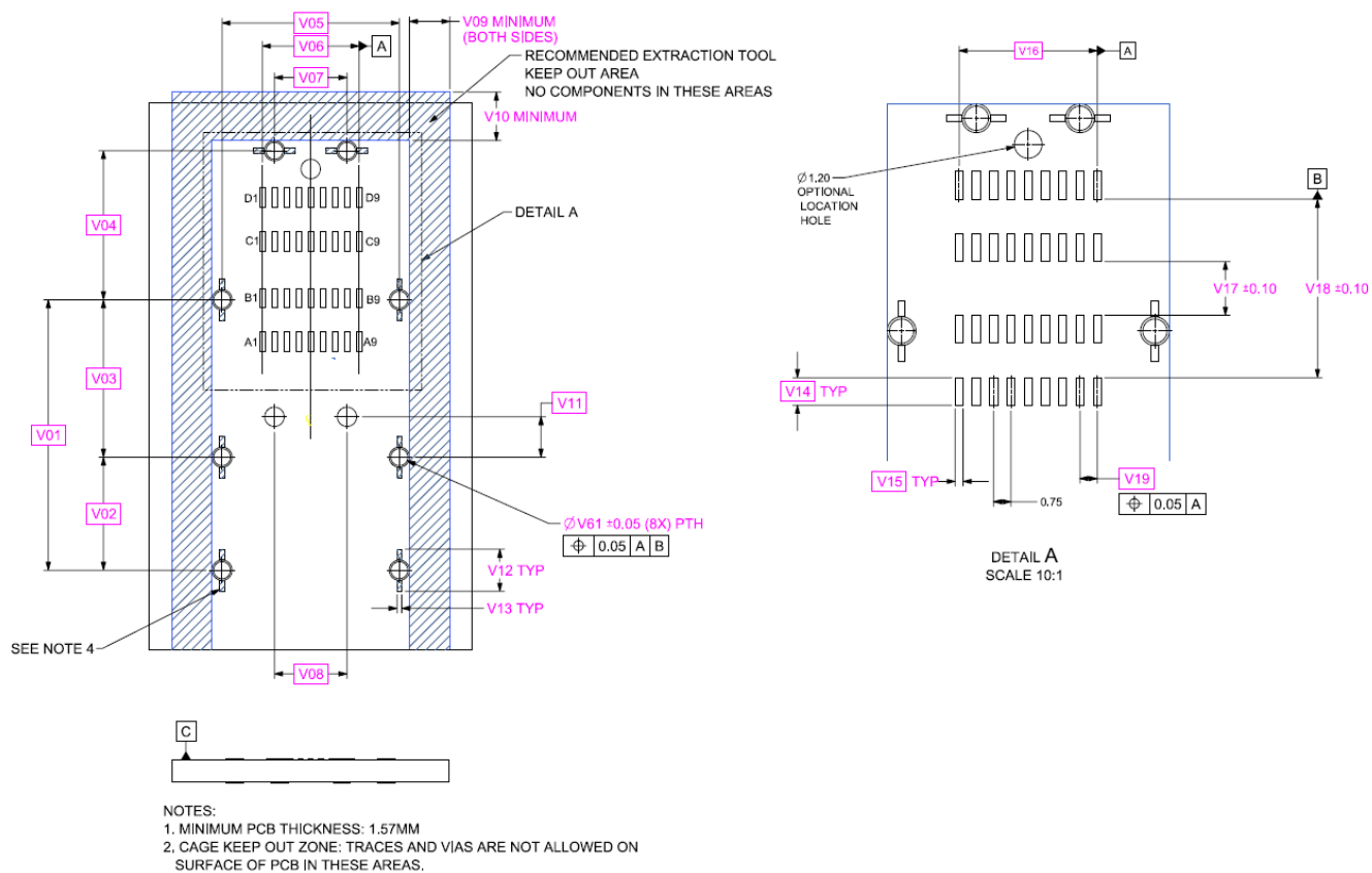
Figure 5-15 1x1 Receptacle SMT Footprint Option
