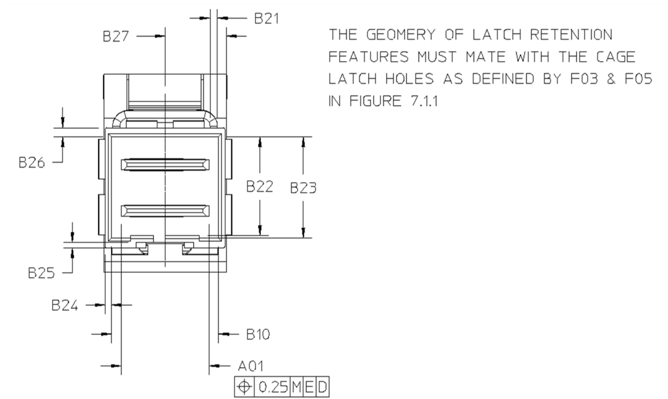
Figure 7-3 4X Plug Retention
