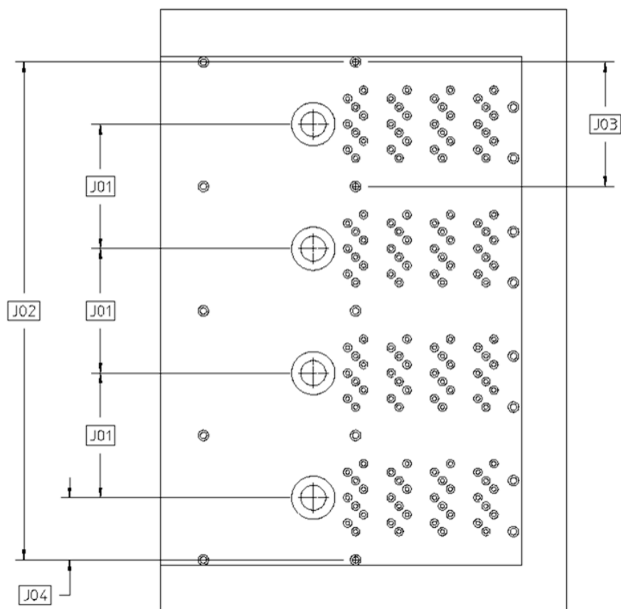
Figure 5-14 1x4 Receptacle Press Fit Footprint Option
