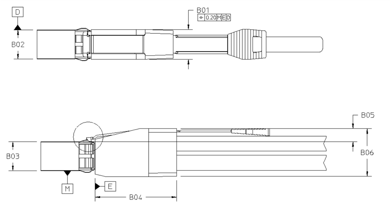
Figure 7-2 4X Plug
