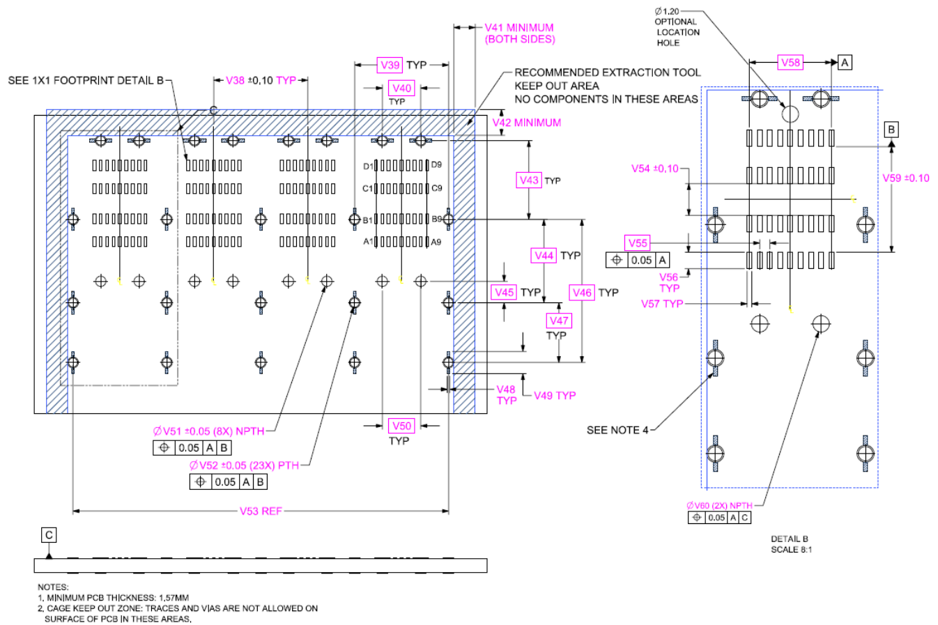
Figure 5-17 1x4 Receptacle SMT Footprint Option
