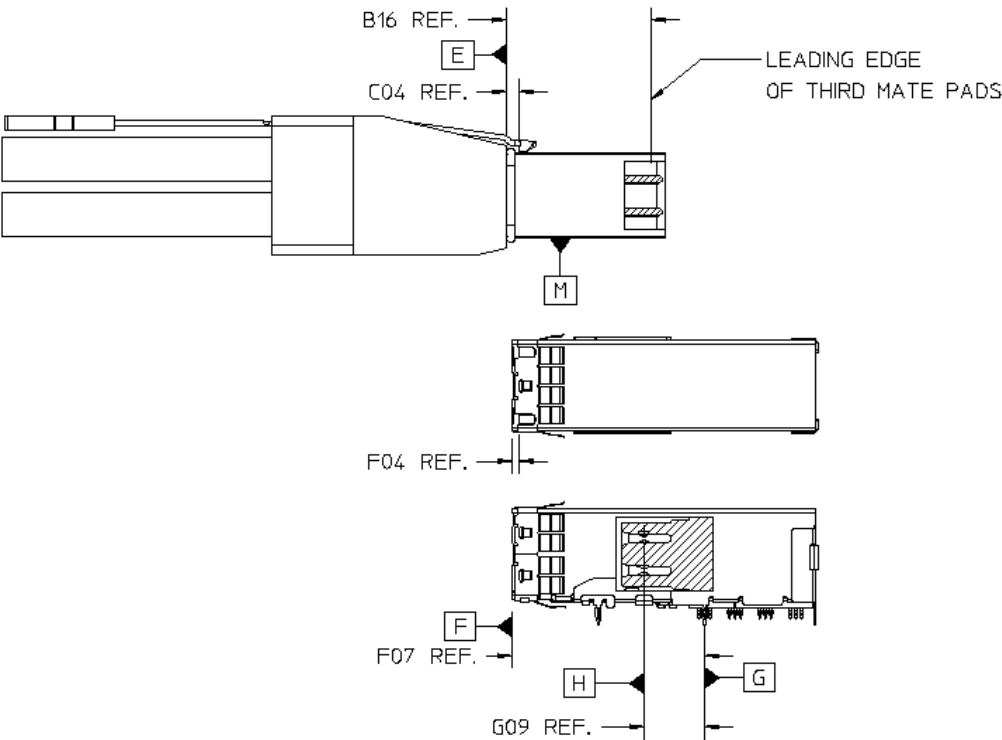
Figure 5-1 Datums (Not All Shown)
