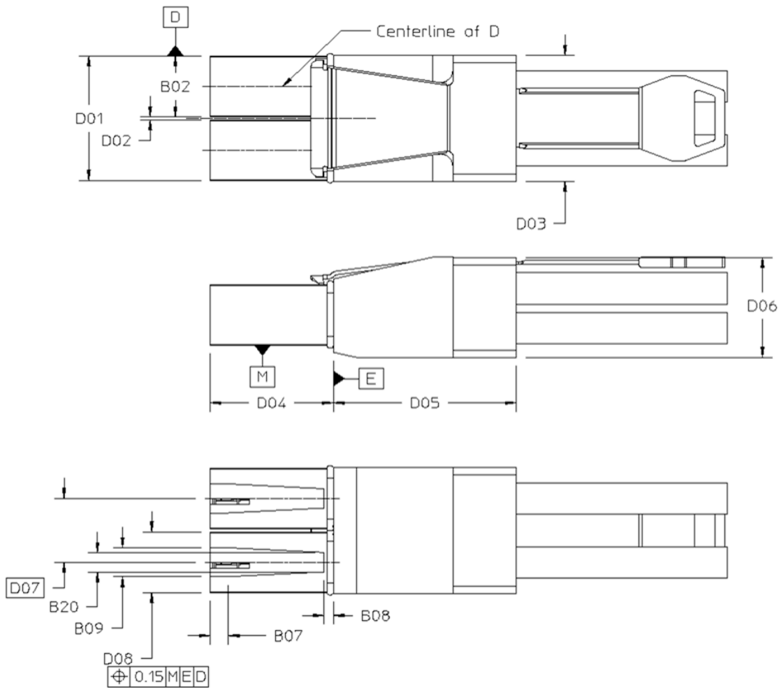
Figure 7-7 8X Plug
