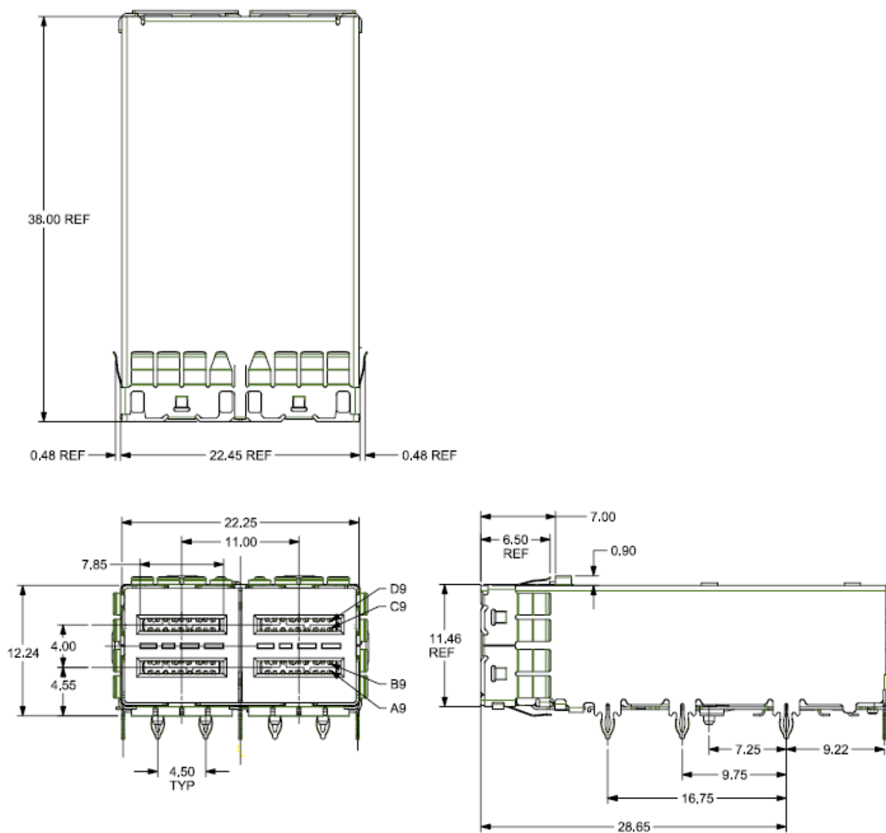
Figure 5-10 Cage for 1x2 SMT Connector
