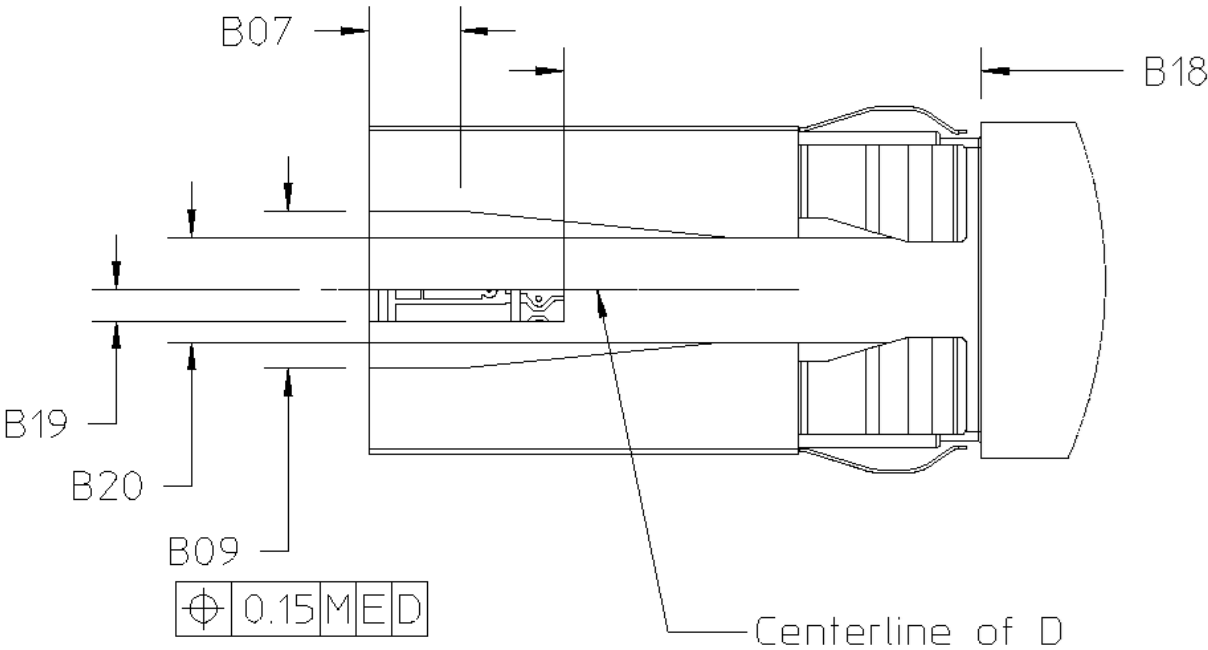
Figure 7-5 4X Plug Key Slot
