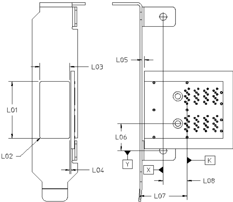
Figure 5-19 1x2 Receptacle to Bezel
