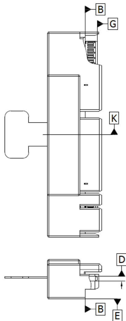
Figure 5-6 Plug Datum Definitions
